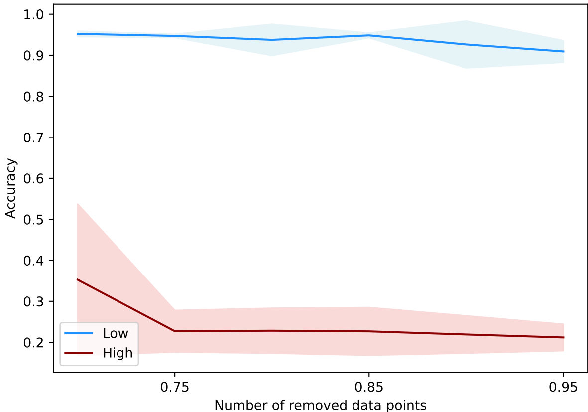
DataAttrOpt(10000, 0.2, 15, best, +b, alpha=best) - bbc-embeddings
